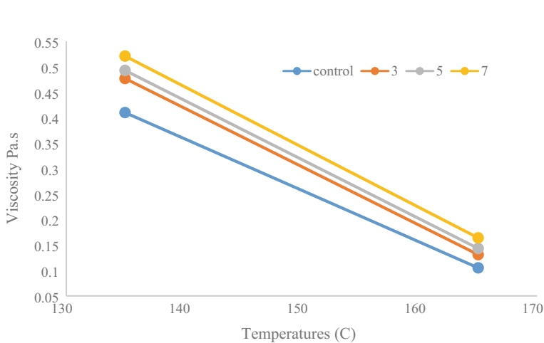
Fig. 4. Base and modified asphalt binder's viscosity
