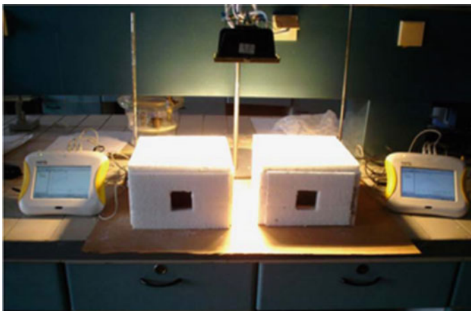
Fig. 5. Polystyrene cubes for thermal performance test [29]
