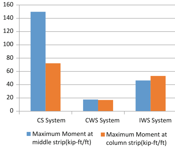
Fig. 2. Demonstrates maximum moment parameter for three distinct type of slabs
